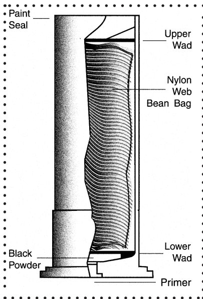
37mm bean bag round
