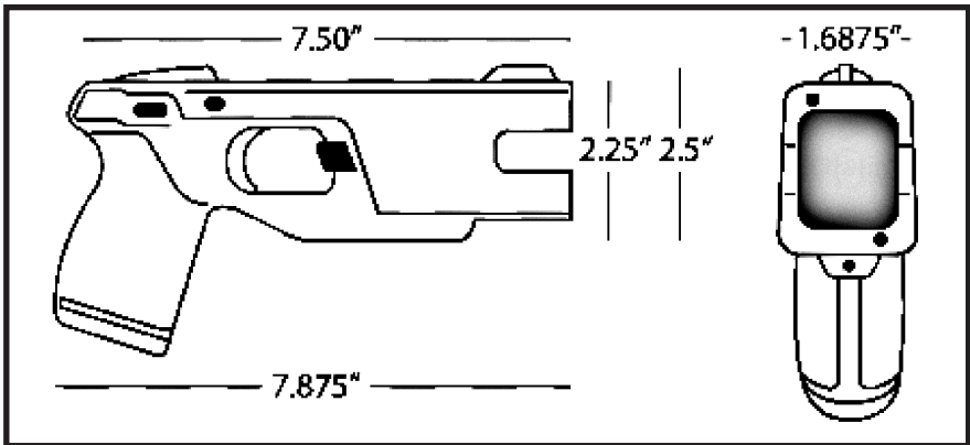
diagram of the TASER Advanced M26
