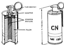
diagram of a tear gas canister
