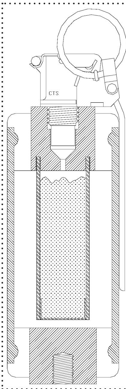
cutaway of non-launchable flash-bang grenade
